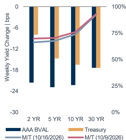
FIGURE 2: MUNIS OUTPERFORMED 2
